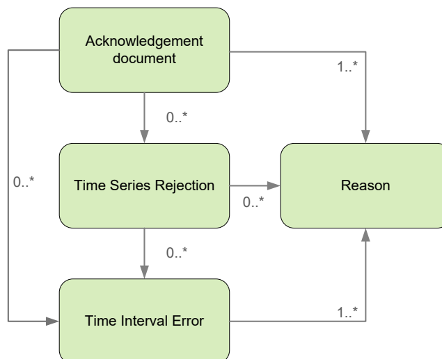
Figure 49 Figure 50 Scheme of Acknowledgement structure
