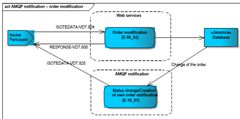
Figure 42 Sending messages scheme – order modification (AMQP notification)
