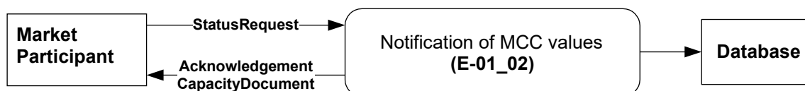
Figure 48 Figure 49 Notification schema of MCC values
