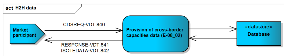
Figure 28 Figure 29 Provision of cross-border capacities scheme
