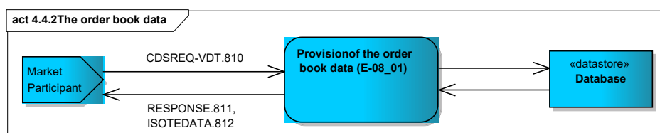
Figure 27 Figure 28 Provision of order book data scheme
