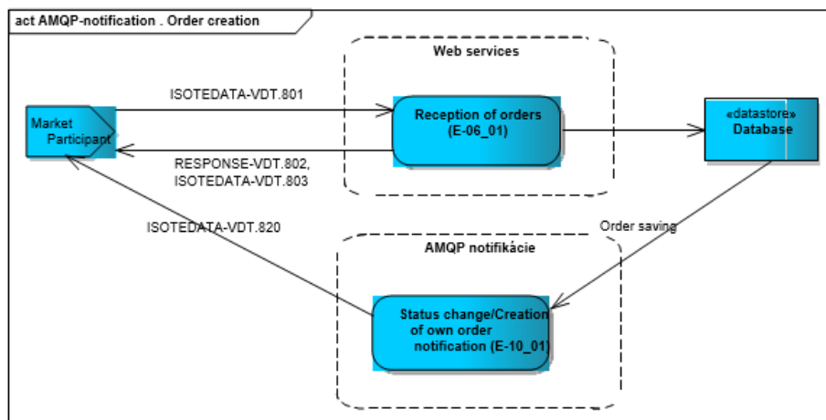
Figure 39 Figure 40 Sending messages scheme – order creation (AMQP notification)
