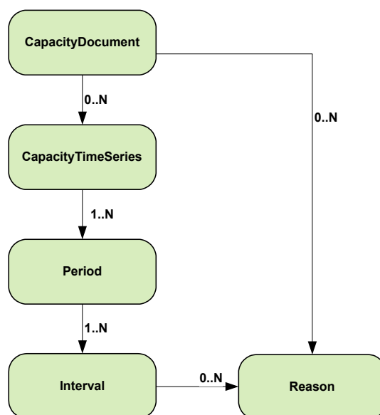
Figure 51 Schema of CapacityDocument structure
