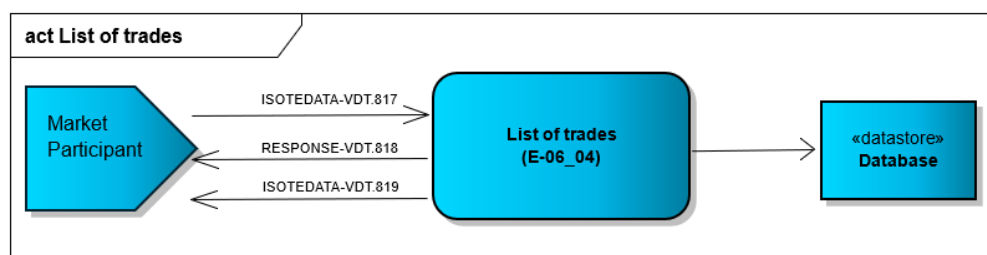
Figure 27 Provision of list of own trades scheme
