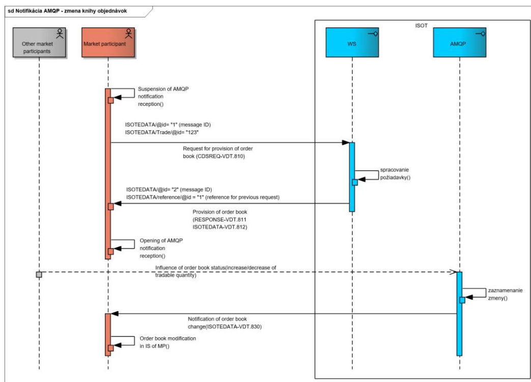
Figure 44 Figure 45 Sequentiality of sent messages scheme – modification of order book (AMQP notification)
