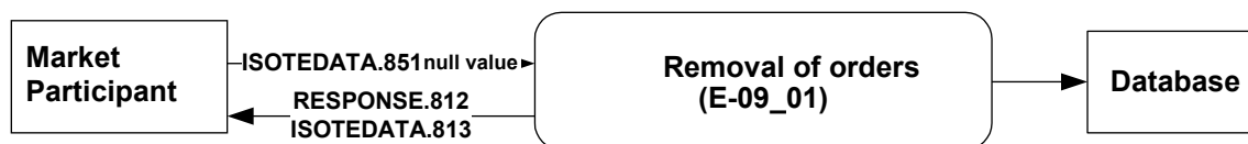
Figure 30 Figure 31 Schema for IDA order removal
