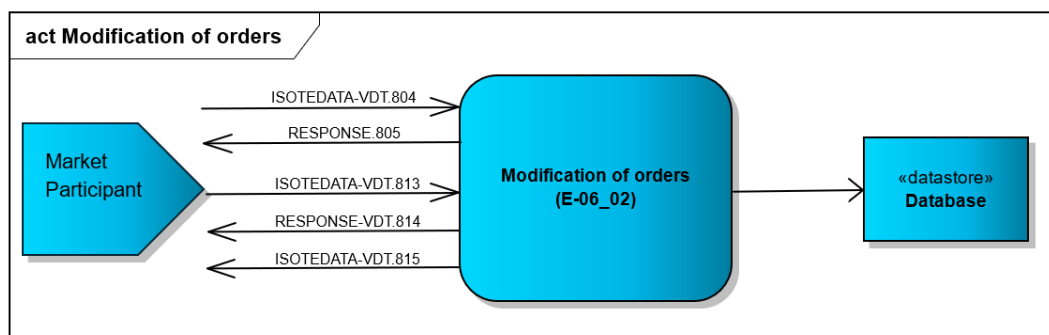
Figure 25 Reception of order scheme
