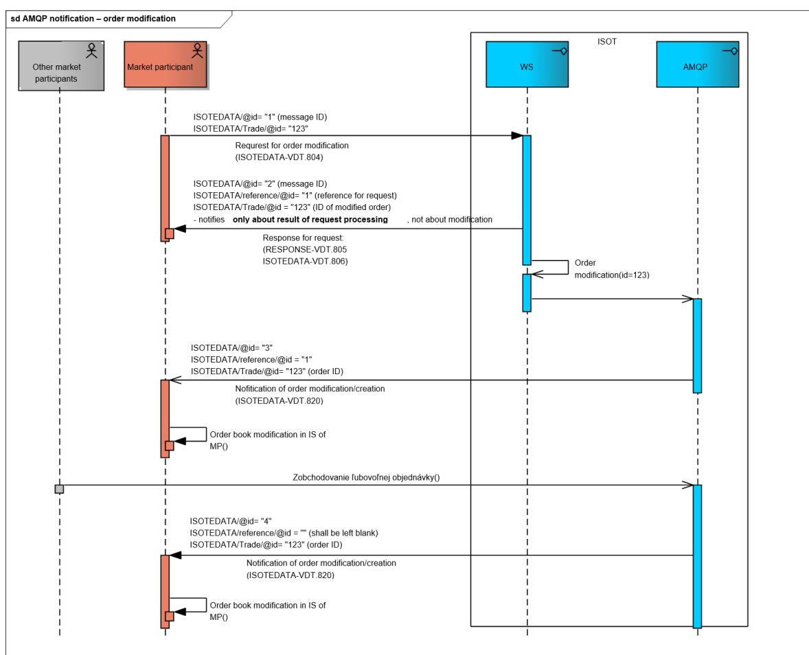
Figure 43 Order of sent messages scheme – order modification (AMQP notification)
